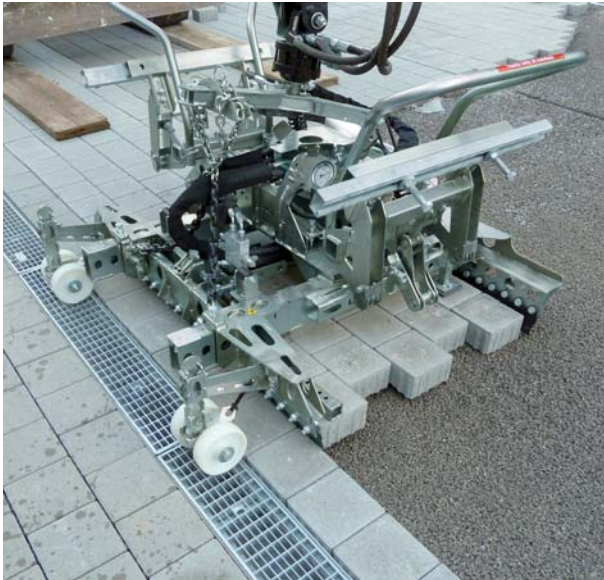
HVZ-ECO Hydraulic Installation Clamp
