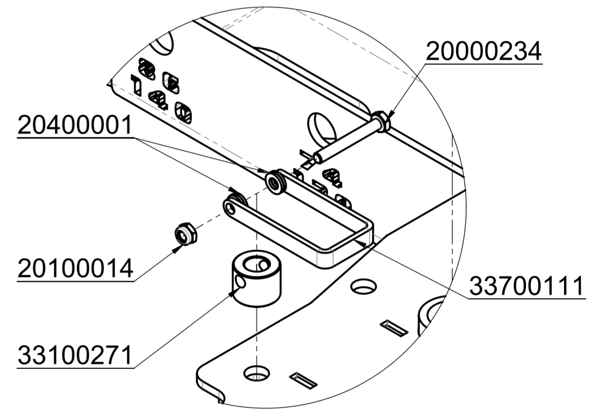
Detail A (1 : 2)
